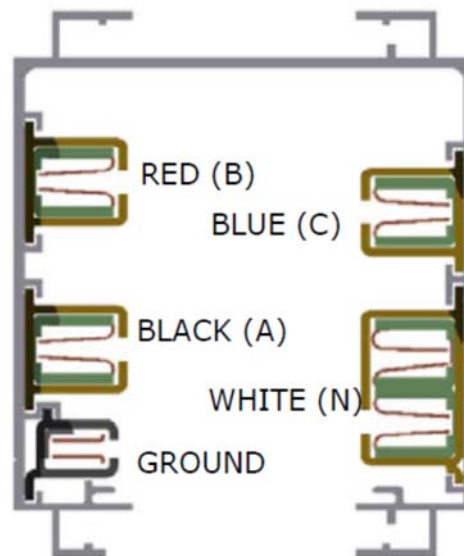
Figure 1: Cross section of a grounded Busway
